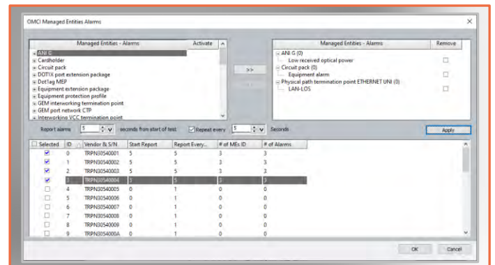
OMCI Alarms and Error Conditions Define OMCI Alarms and Transmission Errors, including Rogue ONU Emulation
