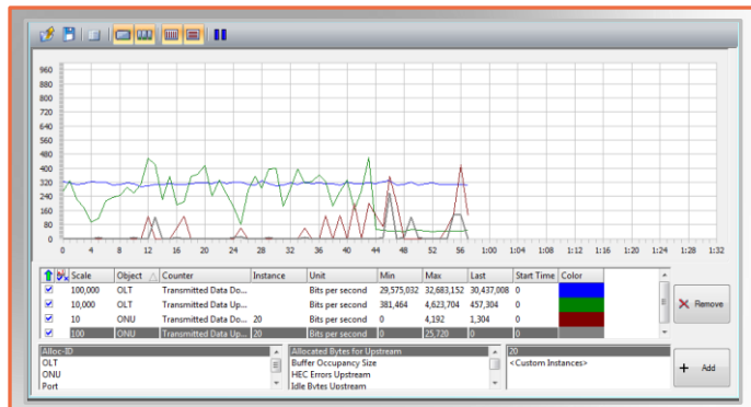
Performance Monitoring Data Rates, Bandwidth Allocations and Error Rates
